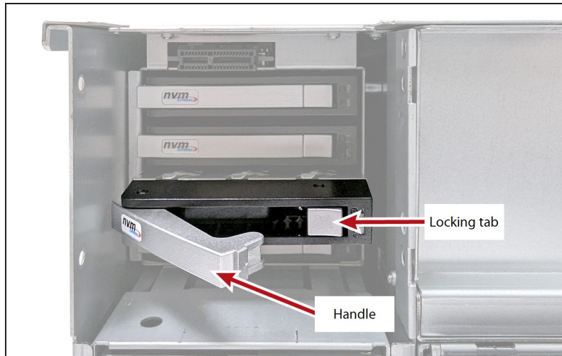
Figure 193 Unlock the drive sled.
